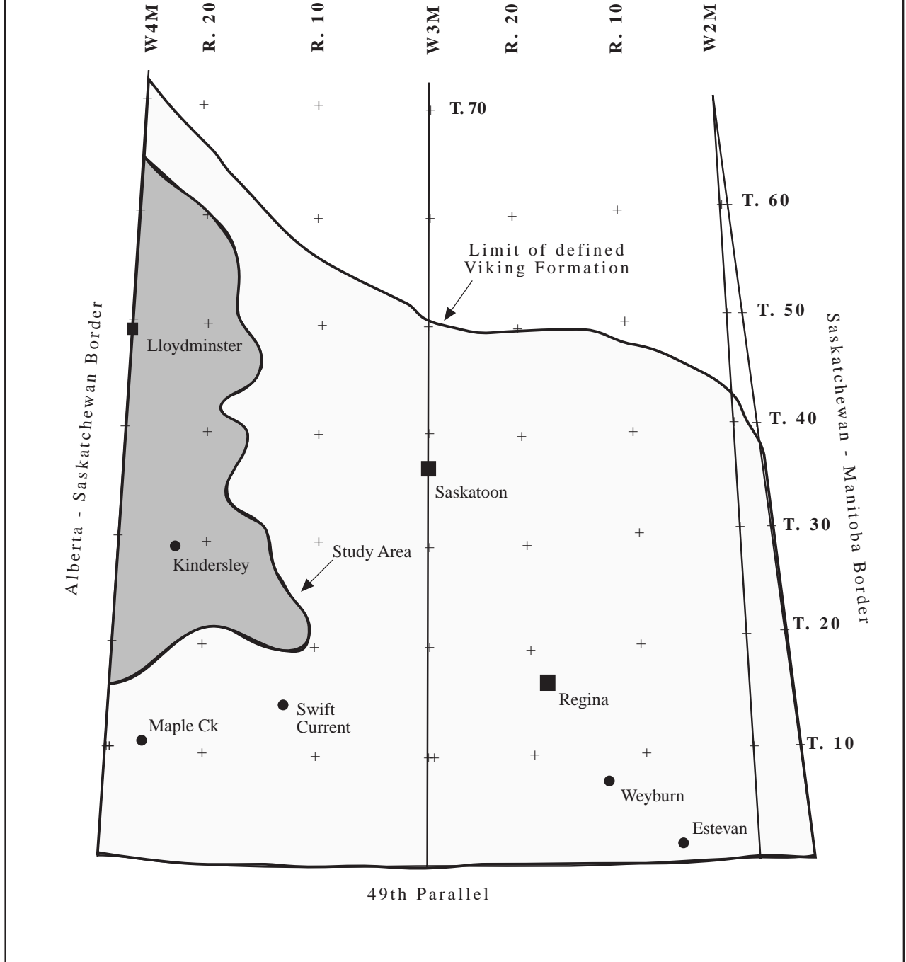
Figure 4 Distribution of the Viking Formation
